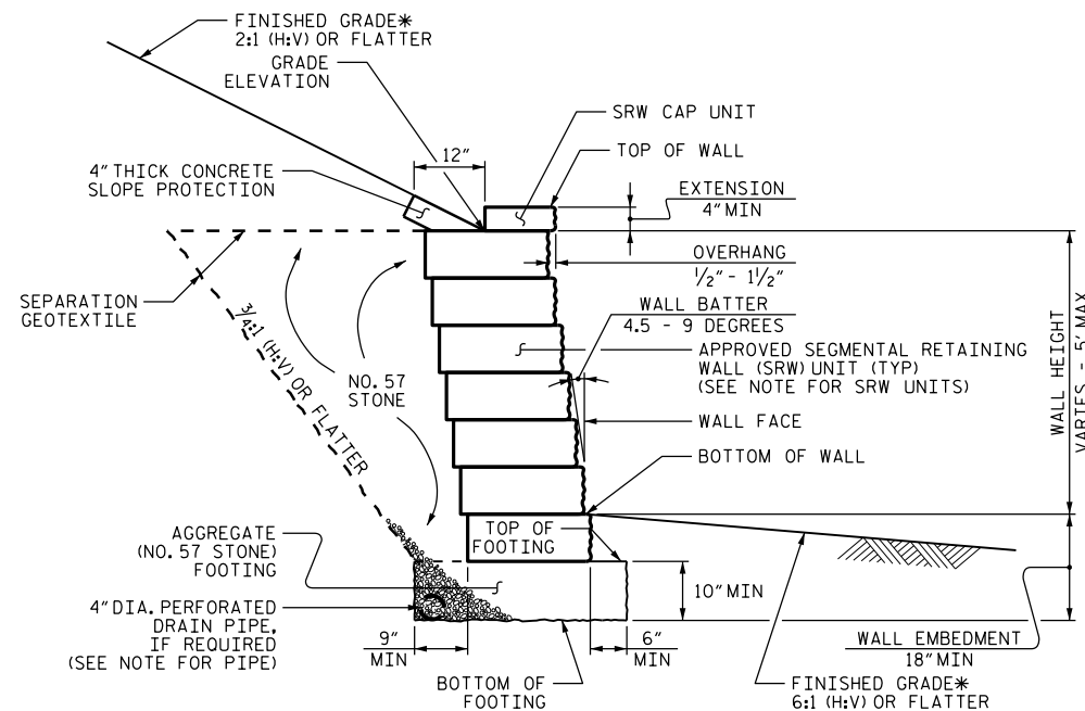
STANDARD SEGMENTAL GRAVITY WALL WITH SLOPE
